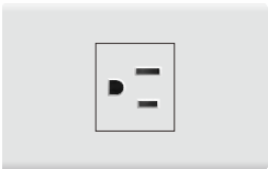
N1-014 1 Gang American socket 15A 125V 16A 250V
